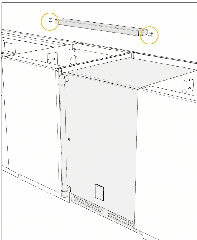
Fig. 10 - Front Countertop Support Spacer
