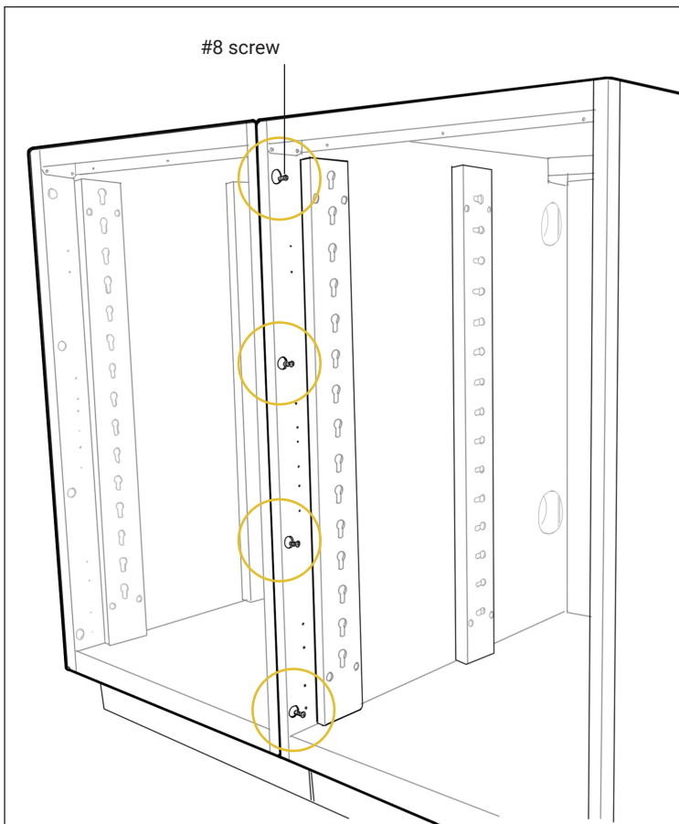
Fig. 2 - Connecting Cabinets FRONTS
