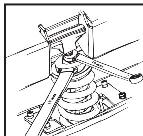
CHARNIÈRE ALTERNATIVE
