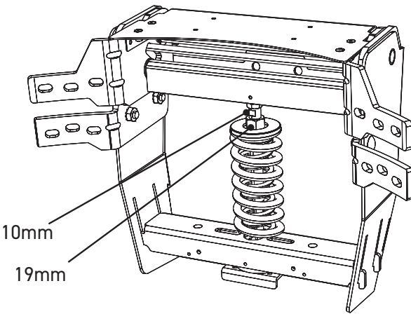
ALTERNATE HINGE
