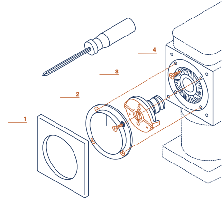
Diagram C: Exploded View
