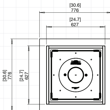
TOP VIEW (Concrete)
