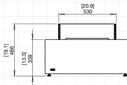
FRONT VIEW (Concrete)
