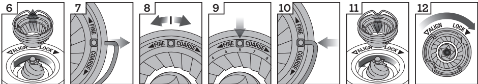
6. Remove upper burr 7. Remove wire handle from both sides of the burr 8. Move adjustable top burr, 1 number, coarser or finer 9. Align the number with the handle opening 10. Insert wire handle into both sides of the burr 11. Push upper burr firmly into position 12. Lock upper burr
